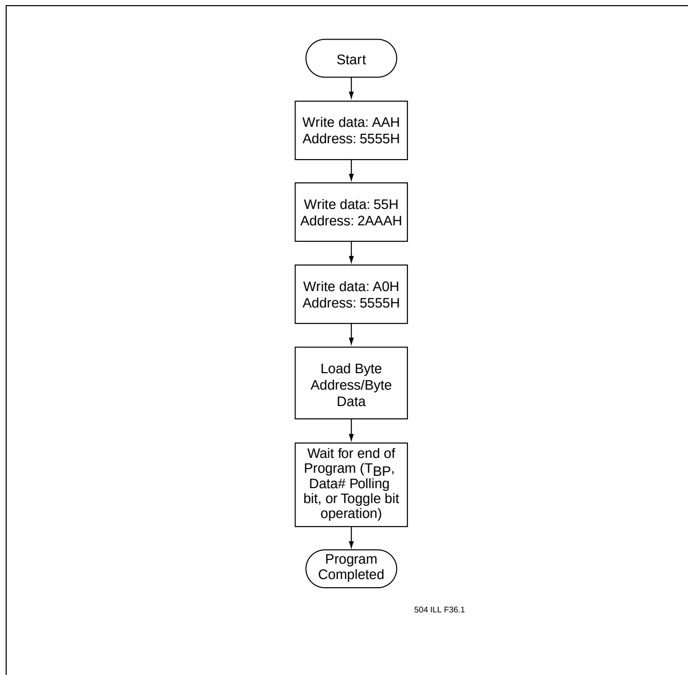
FIGURE 26: BYTE-PROGRAM ALGORITHM
