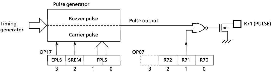
Figure 3-20. Pulse Generator
