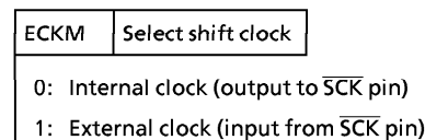
Figure 3-27. Serial Interface Control Command Register
