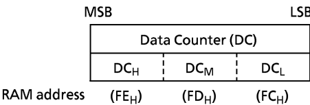
Figure 2-7. Data Counter
