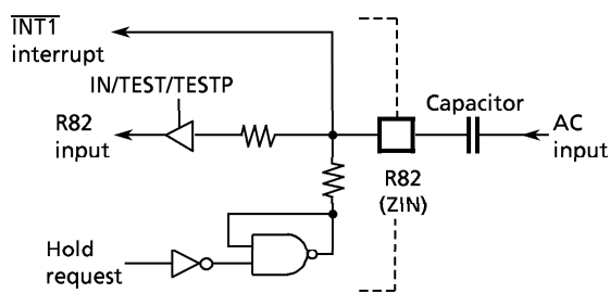
Figure 3-24. Zero-cross Detector
