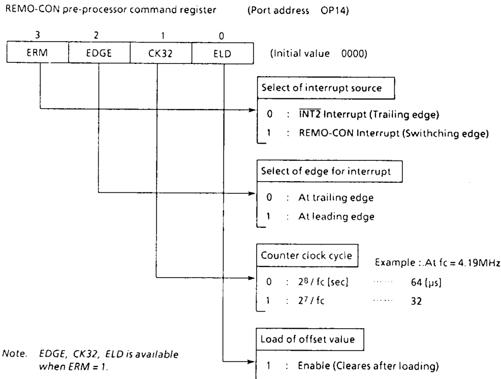
Figure 2-7. Command Register
