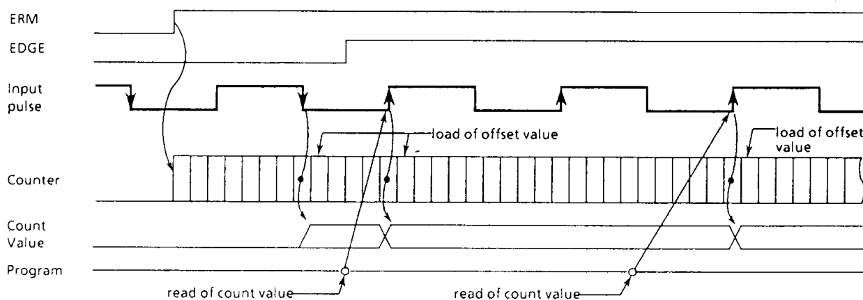
Figure 2-8. Timing chart
