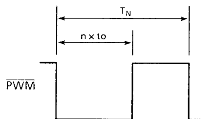
Figure 2-4. \overline{\text{PWM}} output waveform
