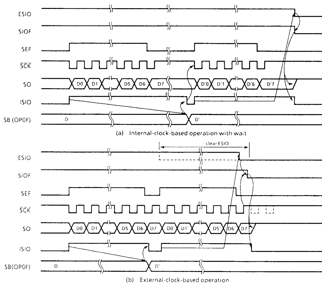
Figure 2-12. 8-bit transmit mode
