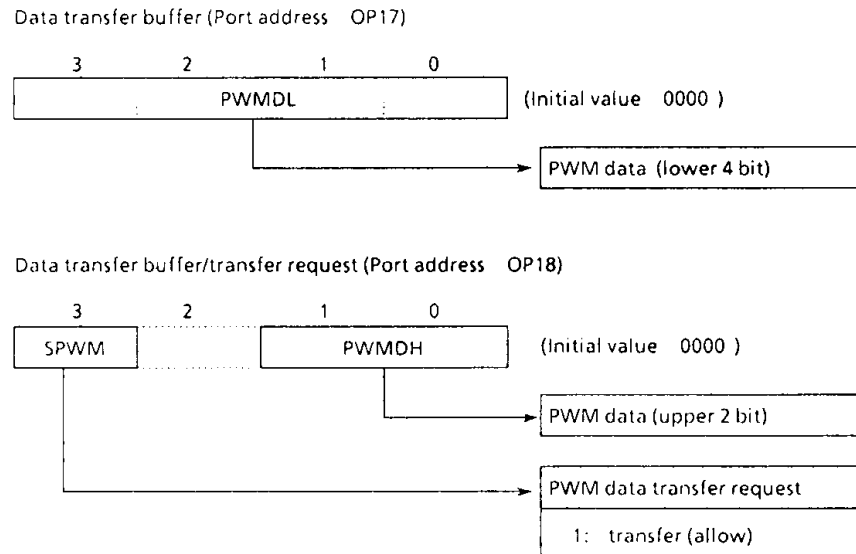
Figure 2-5. Command Register
