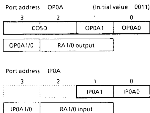
Figure 1. RA Port
