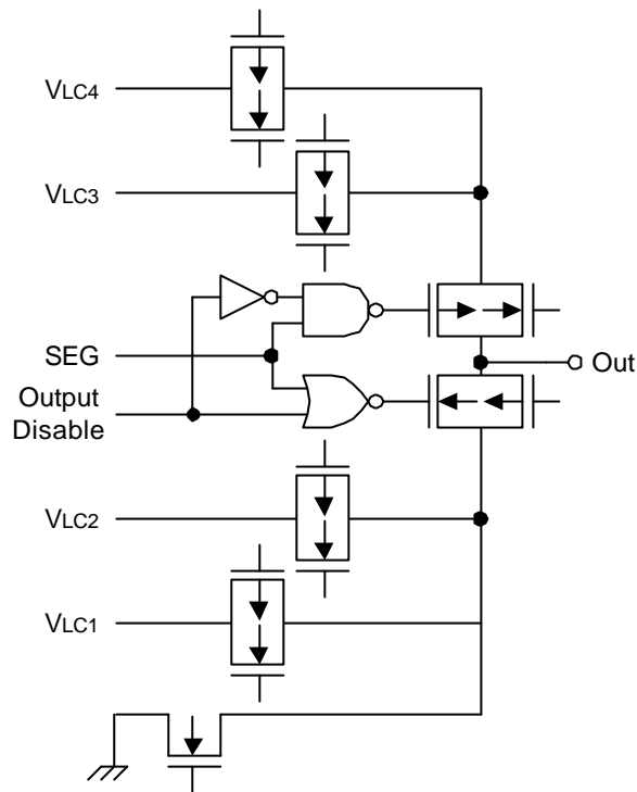
Figure 1-15. Pin Circuit Type H-4
