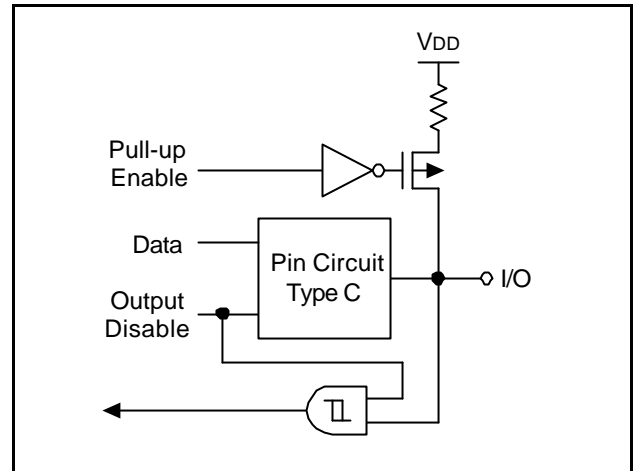
Figure 1-7. Pin Circuit Type D-2
