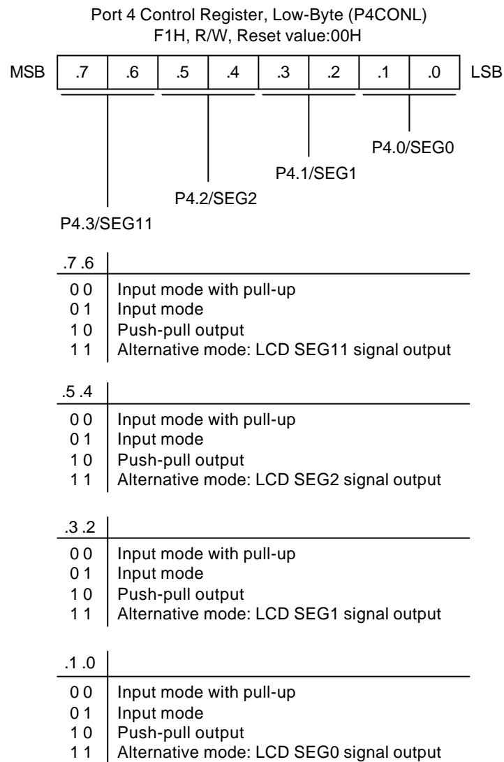
Figure 9-15. Port 4 Low-Byte Control Register (P4CONL)
