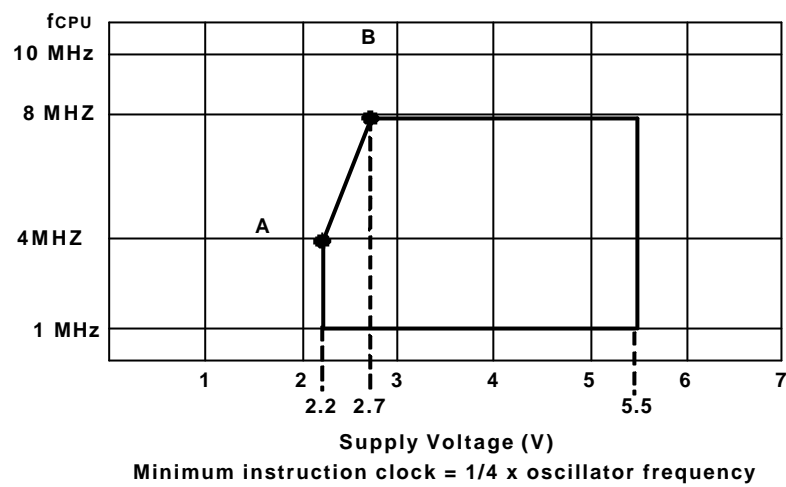
Figure 19-9. Operating Voltage Range
