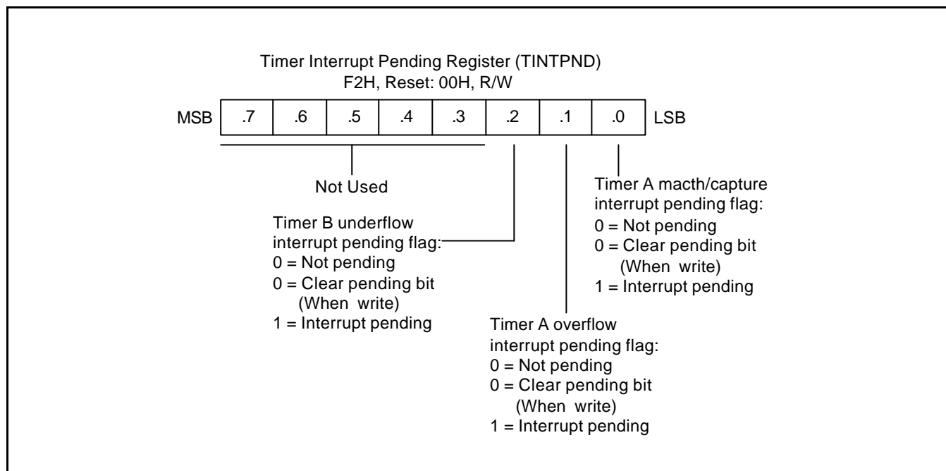
Figure 11-2. Timer interrupts Pending Register (TINTPND)
