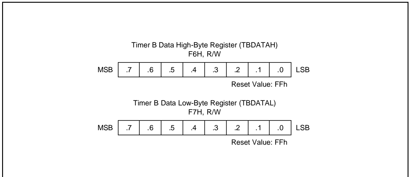
Figure 11-7. Timer B DATA Registers (TBDAHAL, TBDAHAL)
