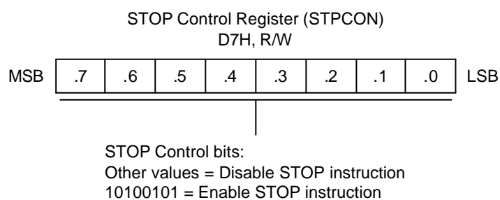
Figure 7-6. STOP Control Register (STPCON)
