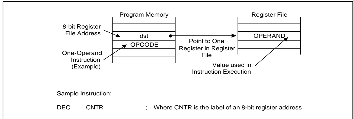
Figure 3-1. Register Addressing
