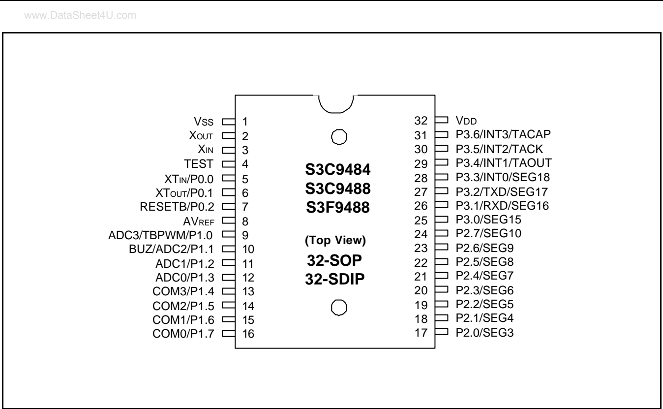
Figure 1-4. S3C9484/C9488/F9488 Pin Assignment (32-SOP/SDIP)
