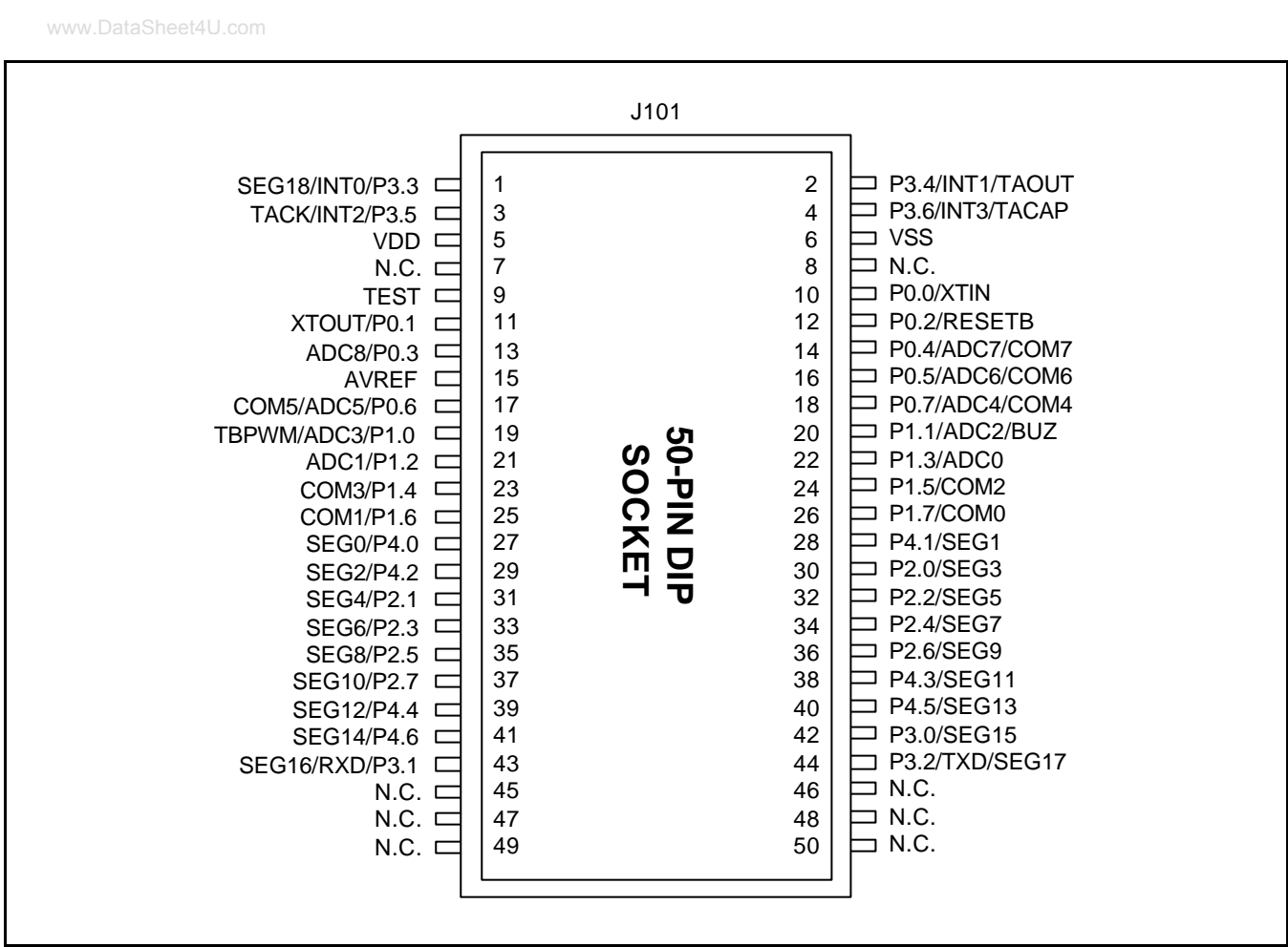
Figure 22-4. 44-Pin Connector for TB9484/88
