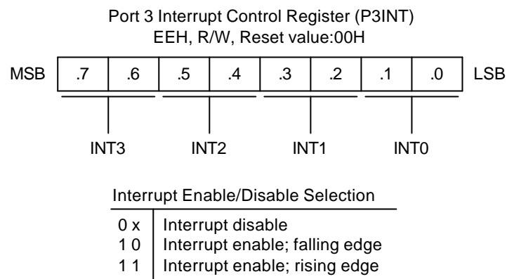
Figure 9-12. Port 3 Interrupt Control Register (P3INT)
