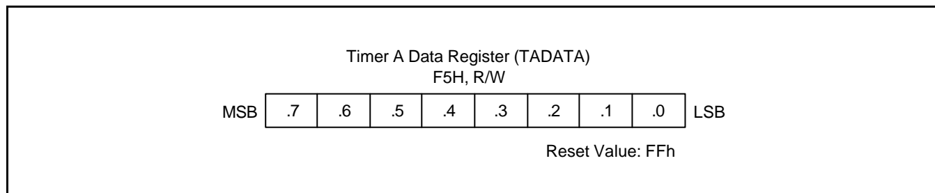
Figure 11-3. Timer A DATA Register (TADATA)
