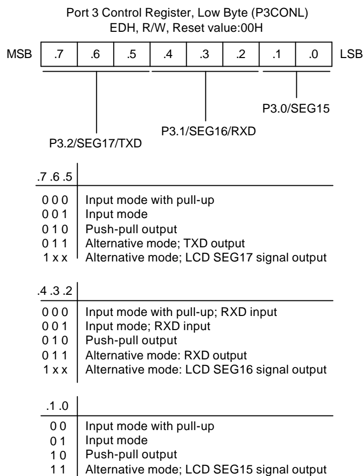
Figure 9-10. Port 3 Low-Byte Control Register (P3CONL)
