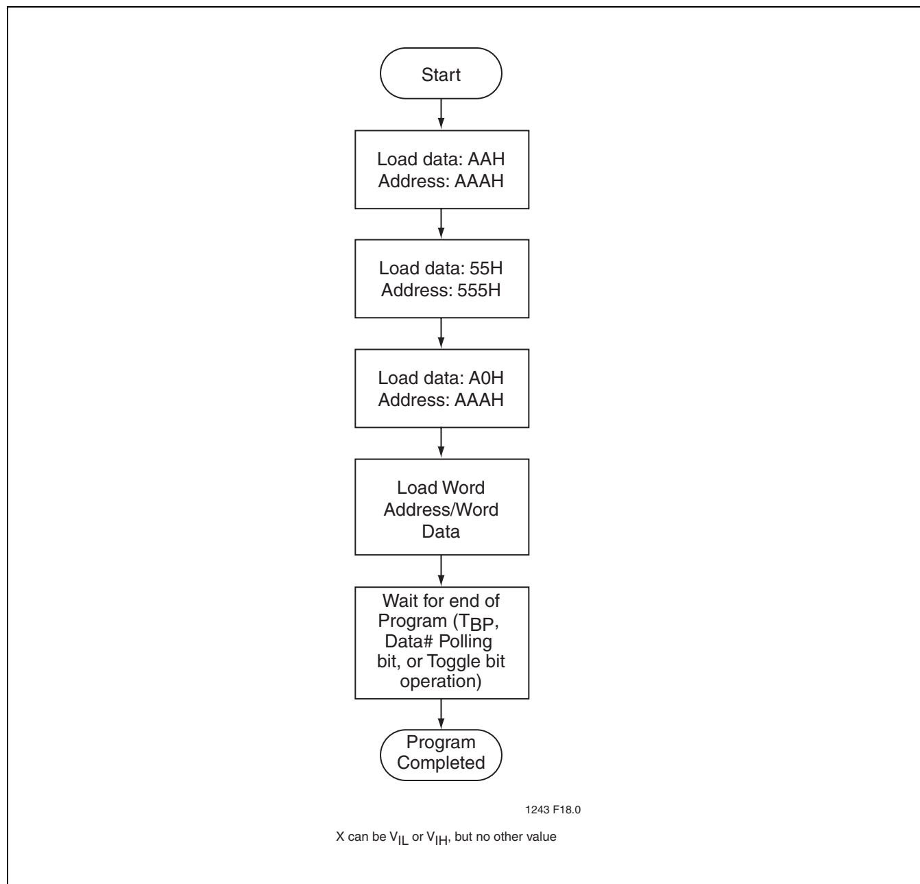
FIGURE 19: BYTE-PROGRAM ALGORITHM
