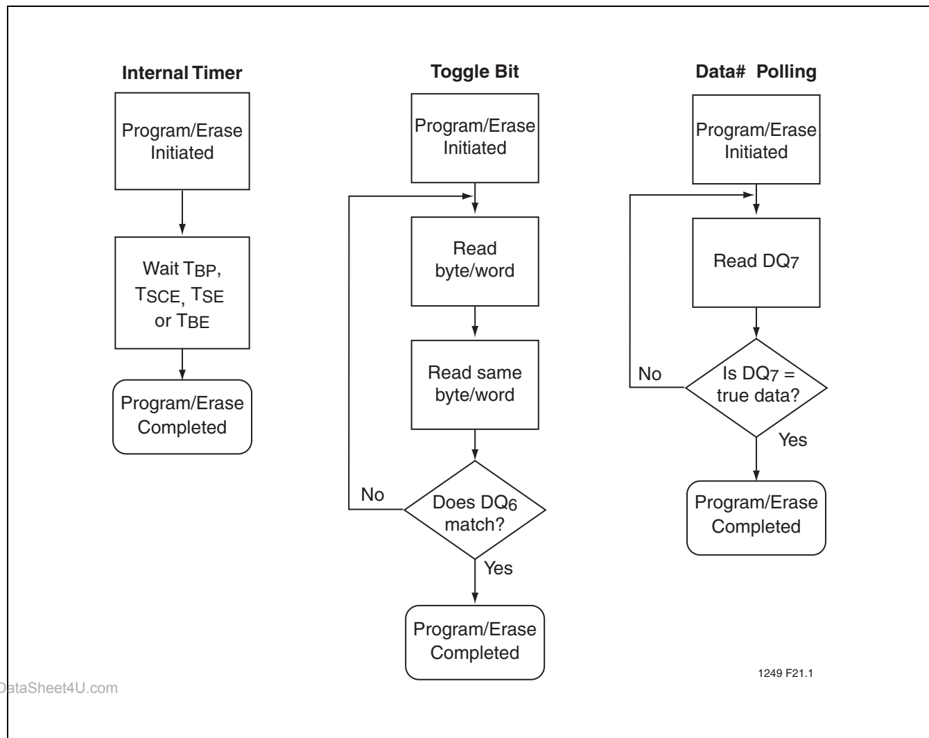
FIGURE 24: WAIT OPTIONS
