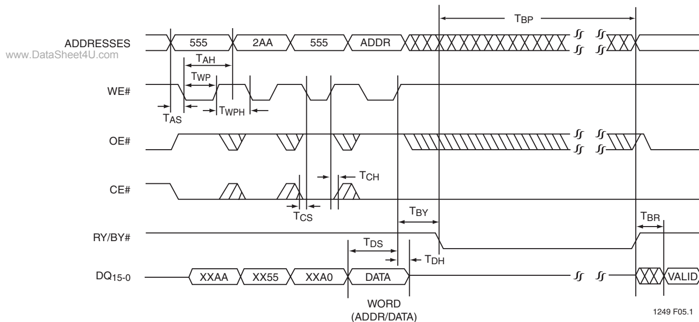
FIGURE 8: WE# CONTROLLED PROGRAM CYCLE TIMING DIAGRAM
