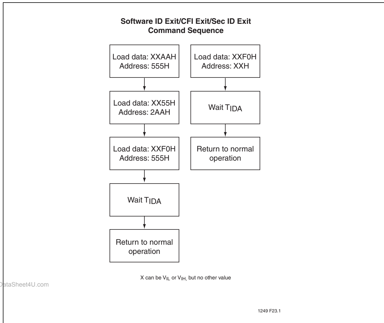
FIGURE 26: SOFTWARE PRODUCT ID/CFI/SEC ID EXIT COMMAND FLOWCHARTS
