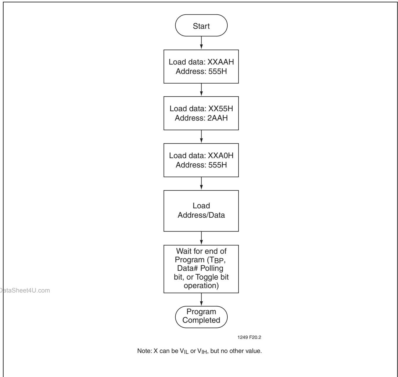
FIGURE 23: PROGRAM ALGORITHM
