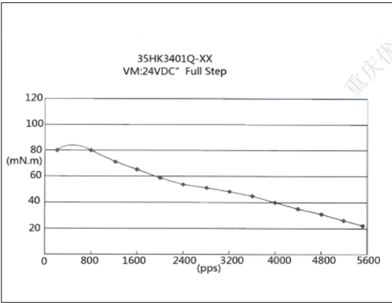
力矩曲线 Torque Curve
