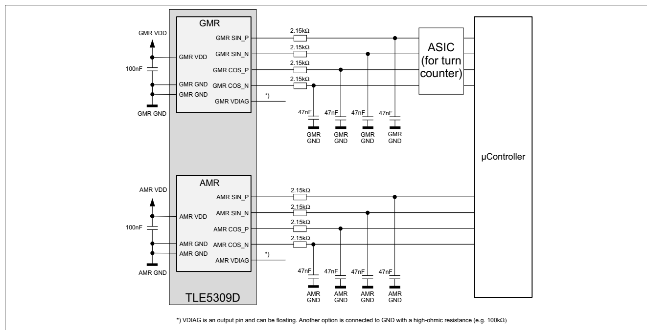
Figure 14 Application circuit for the TLE5309D in low-power applications in differential output mode (e.g. turn counter)
