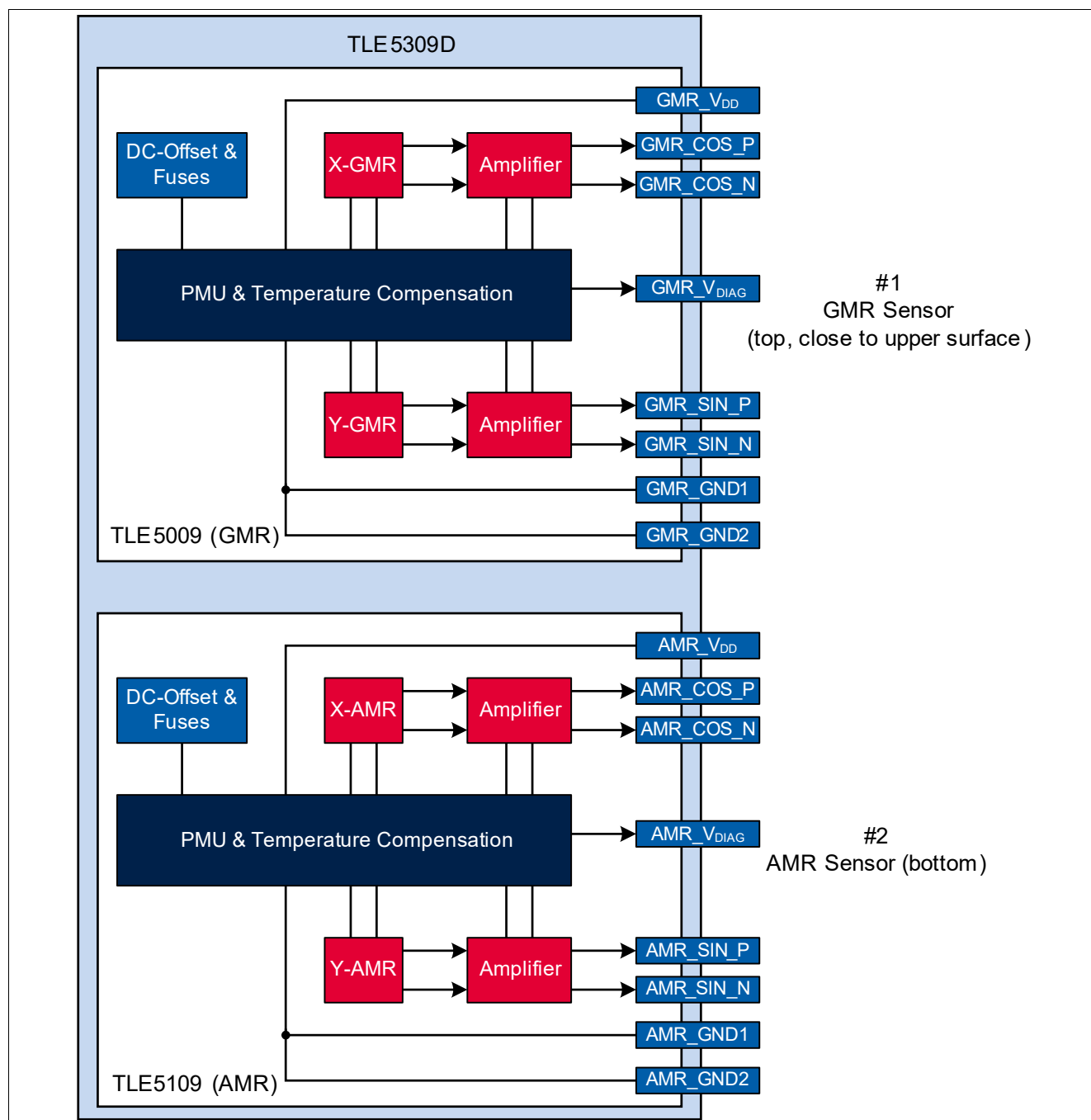
Figure 7 TLE5x09A16(D) block diagram example: TLE5309D sensor with die 1 GMR- and die 2 AMR-sensing technology
