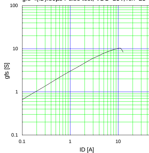
Typical Transconductance
