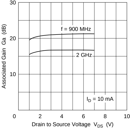
Associated Gain vs. Drain to Source Voltage
