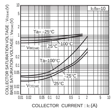
Fig.6 Collector-emitter saturation vs. collector current
