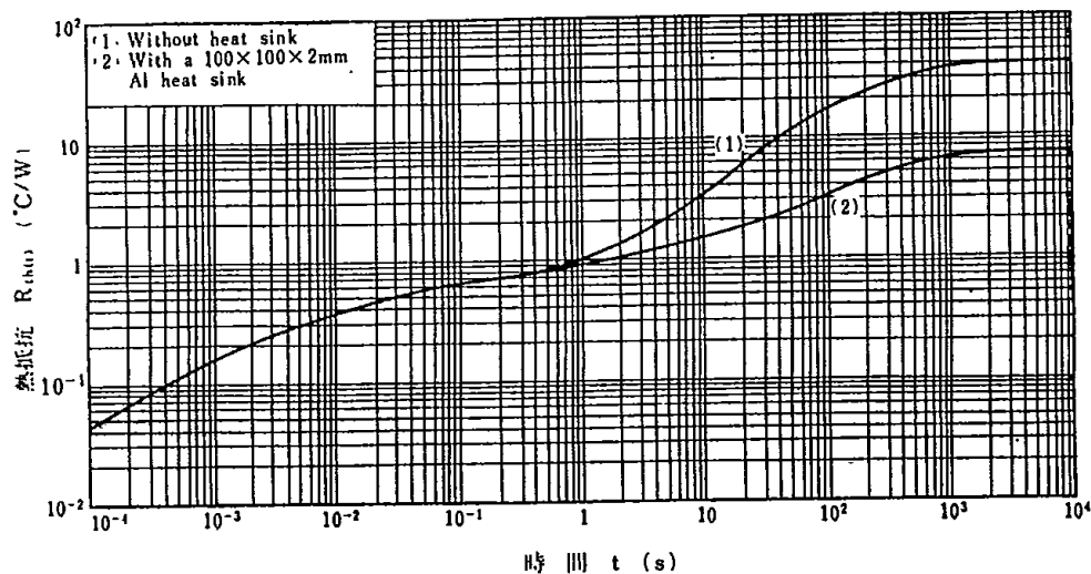
R_{th(t)} - t
