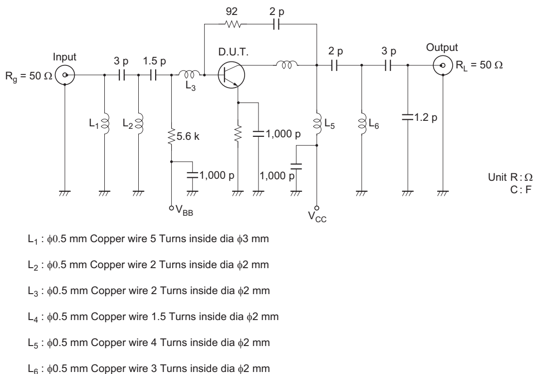
Circuit Example-UHF Wide Bandwidth Amplifier ( f = 500\text{ MHz to }950\text{ MHz} )
