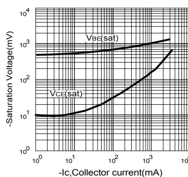
Fig.8 Saturation Voltage
