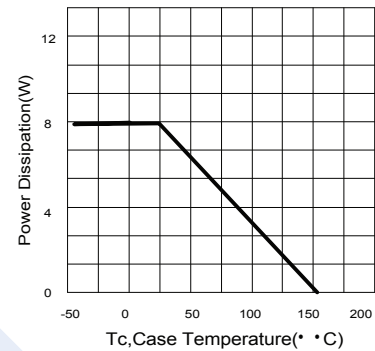
Fig.3 Power Derating
