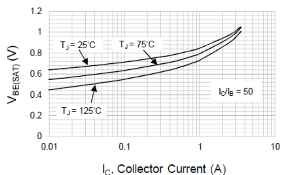
Fig.1 Typical Base-Emitter Saturation Voltage
