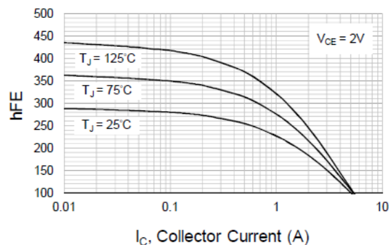
Fig.5 Typical DC Current Gain vs Collector Current
