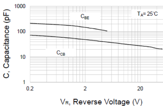
Fig.6 Typical Capacitance
