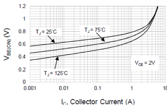
Fig.2 Typical Base-Emitter Saturation Voltage
