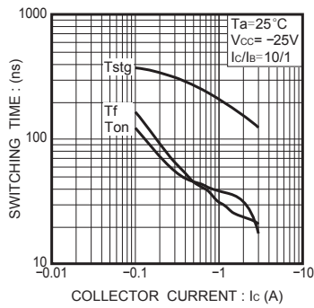
Fig.1 Switching Time
