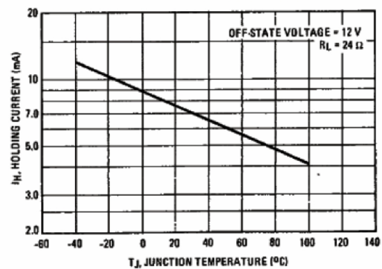
HOLDING CURRENT
