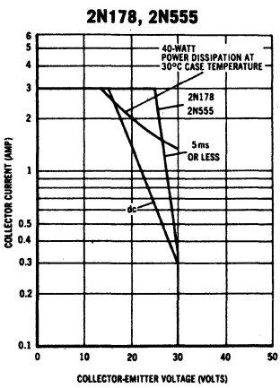
SAFE OPERATING AREAS
