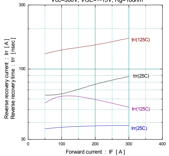
[ Inverter ] Reverse recovery characteristics (typ.) Vcc=300V, VGE=+-15V, Rg=16ohm
