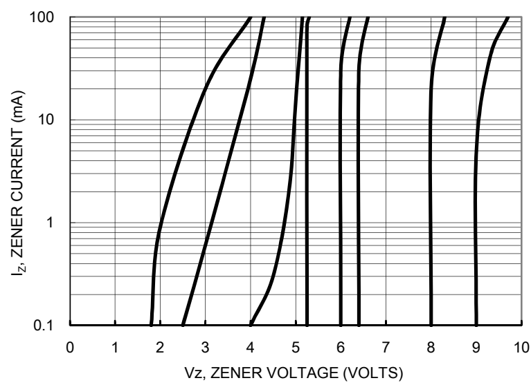
FIG. 6- Vz = 6.8 - 10 VOLTS
