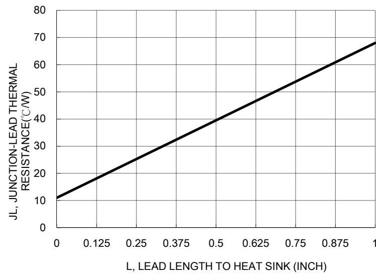
FIG. 9- TYPICAL THERMAL RESISTANCE
