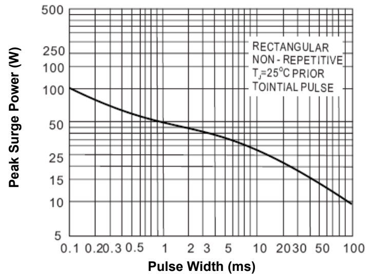
Fig.1-Max.Surge Power
