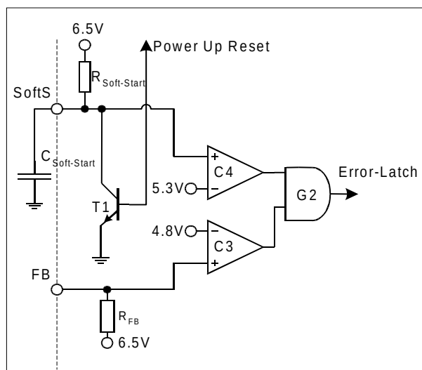
Figure 20 FB-Detection
