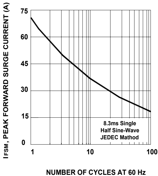
Fig.3 Max Non-Repetitive Peak Forward Surge Current
