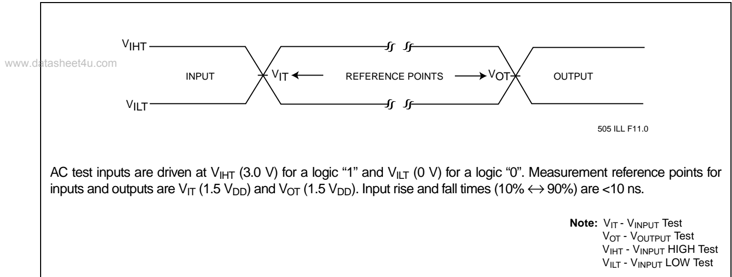
FIGURE 13: AC INPUT/OUTPUT REFERENCE WAVEFORMS FOR SST29SFxxx
