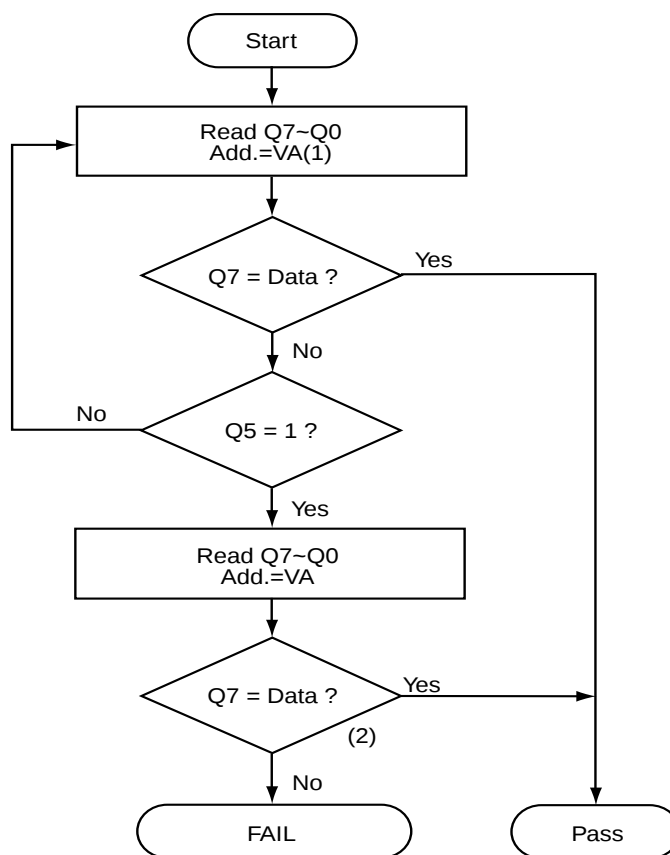
Figure 18. DATA POLLING ALGORITHM
