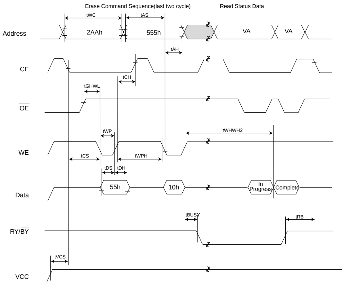
Figure 6. AUTOMATIC CHIP ERASE TIMING WAVEFORM
