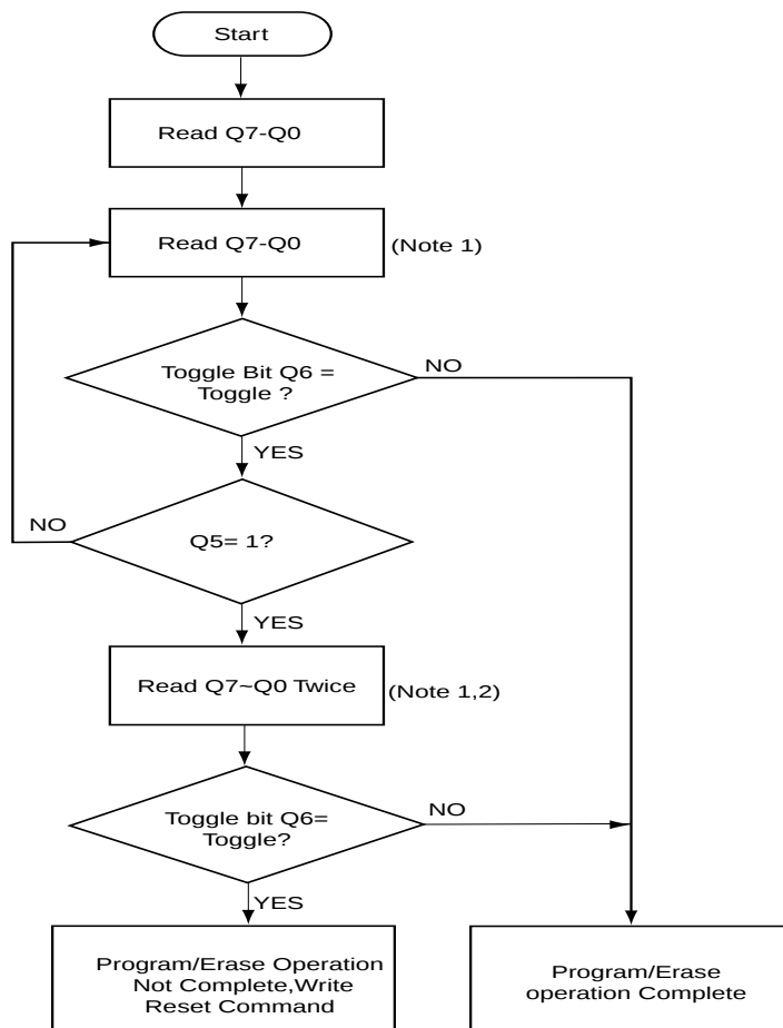
Figure 19. TOGGLE BIT ALGORITHM
