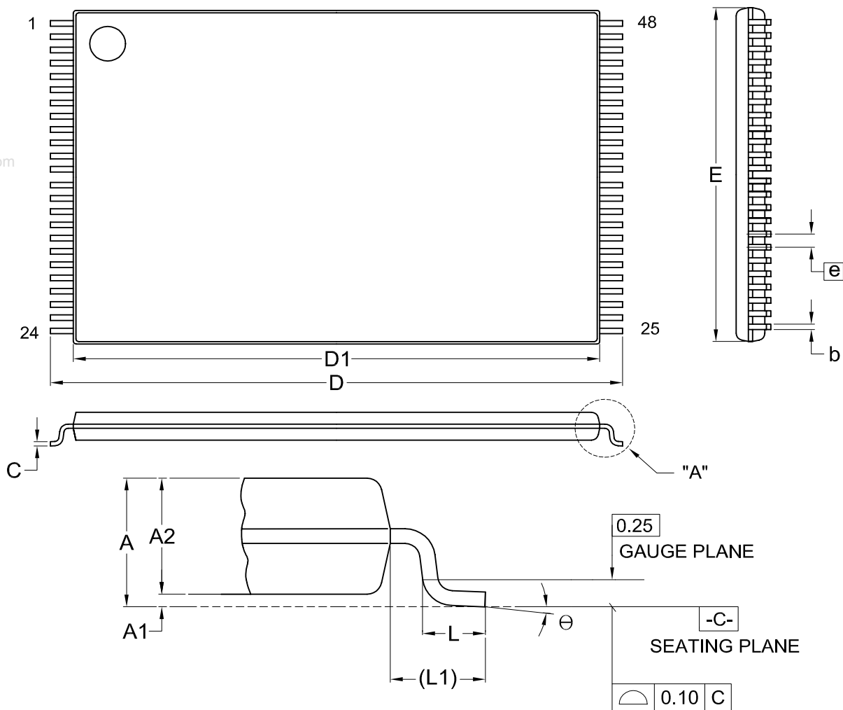
DETAIL "A"
