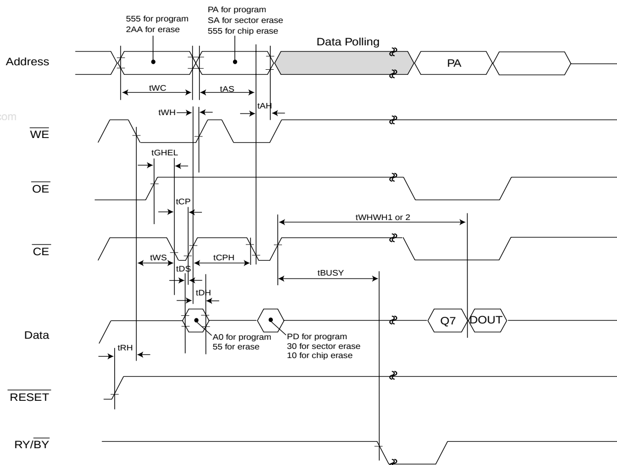
Figure 5. \overline{\text{CE}} CONTROLLED WRITE TIMING WAVEFORM
