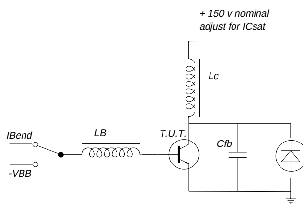
Fig.5. Switching times test circuit.
