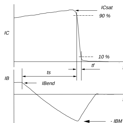
Fig.4. Switching times definitions.
