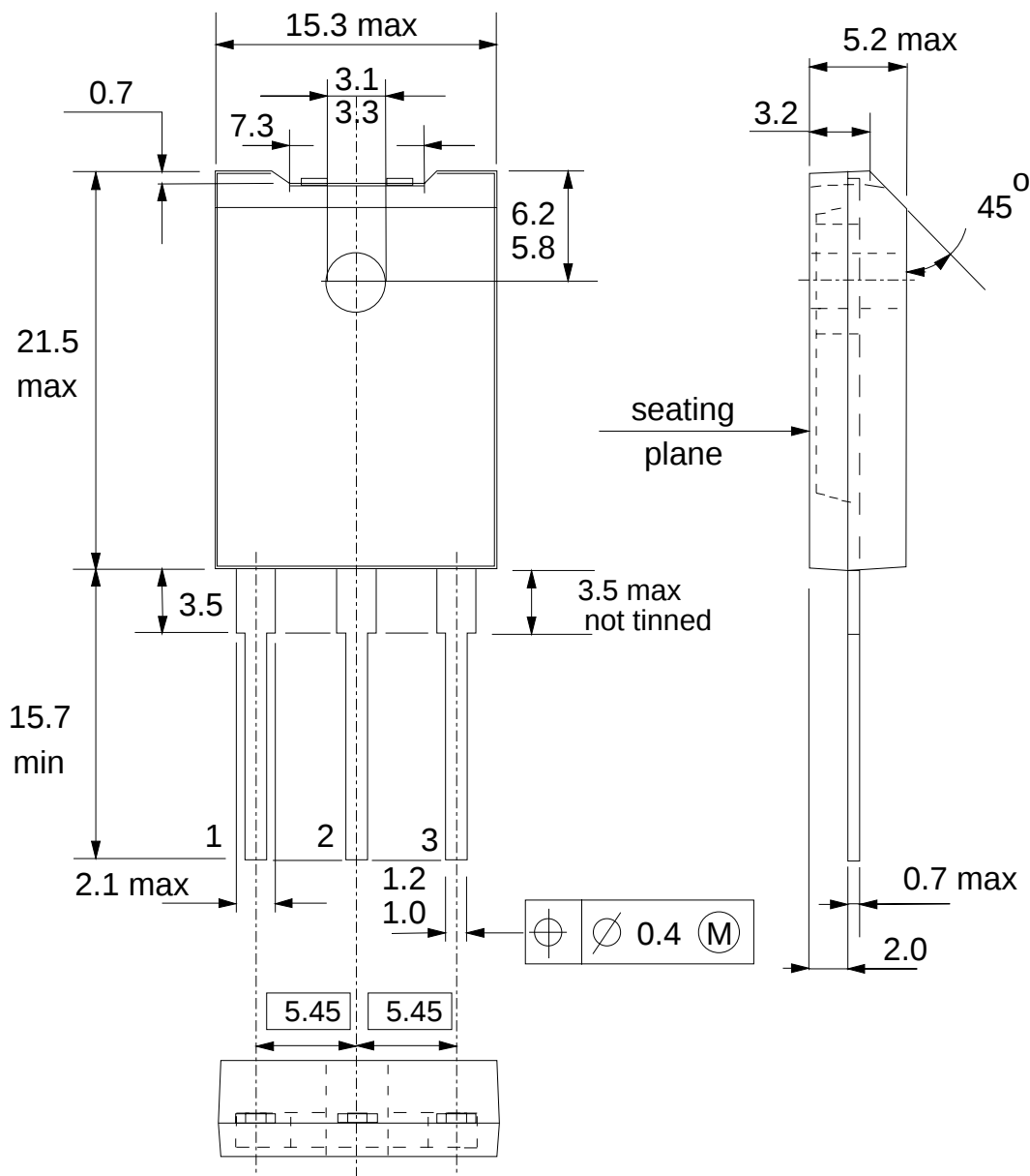
Fig.17. SOT199; The seating plane is electrically isolated from all terminals.
