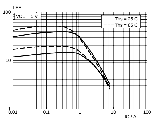
Fig.6. DC current gain. h_{FE} = f(I_C) Parameter T_{hs} (Low and high gain)
