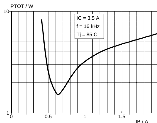
Fig.10. Limit P_{tot} ; T_J = 85^\circ\text{C} P_{tot} = f(I_{B(end)}) ; I_C = 3.5\text{ A} ; f = 16\text{ kHz}
