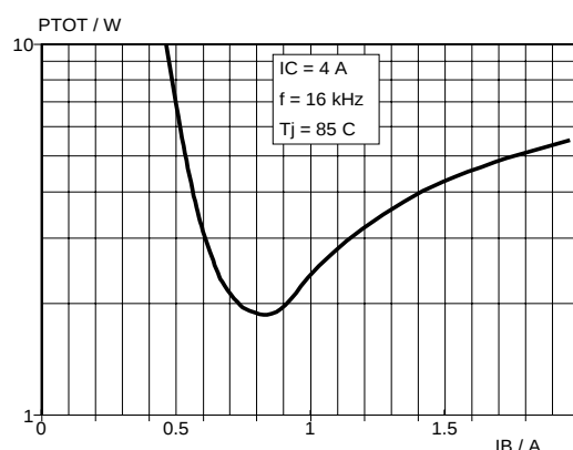
Fig.11. Limit P_{tot} ; T_J = 85^\circ\text{C} P_{tot} = f(I_{B(end)}) ; I_C = 4.0\text{ A} ; f = 16\text{ kHz}
