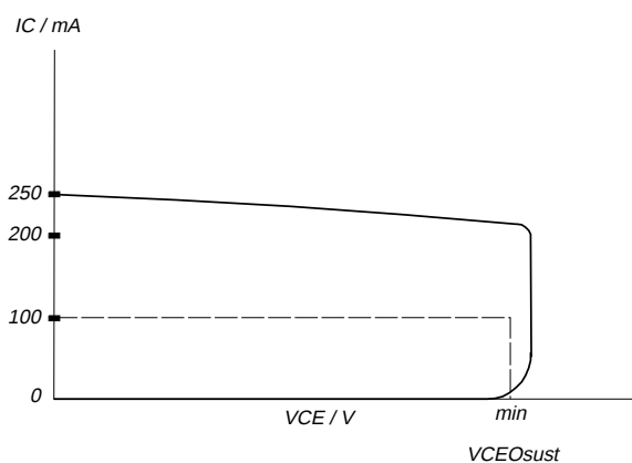
Fig.2. Oscilloscope display for V_{CEOsust} .
