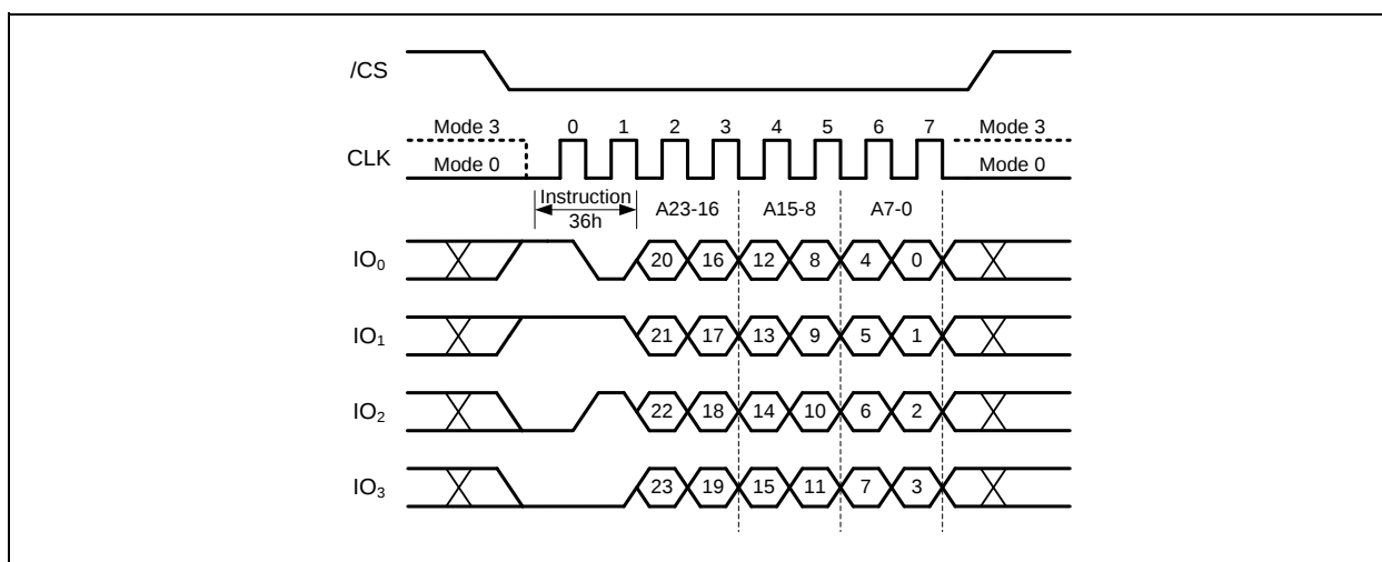
Figure 51b. Individual Block/Sector Lock Instruction (QPI Mode)
