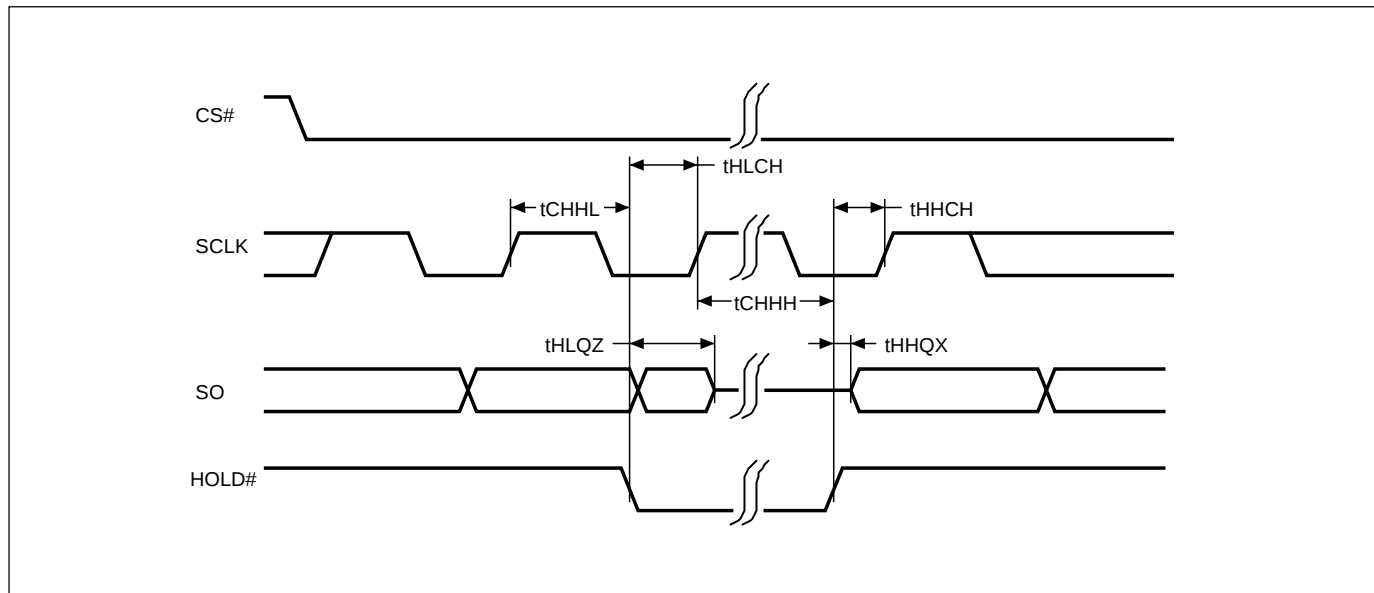
Figure 10. Hold Timing
