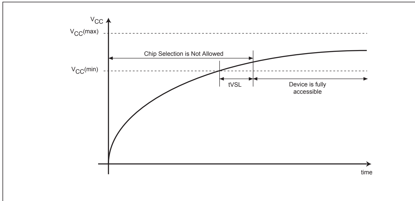
Figure 26. Power-up Timing
