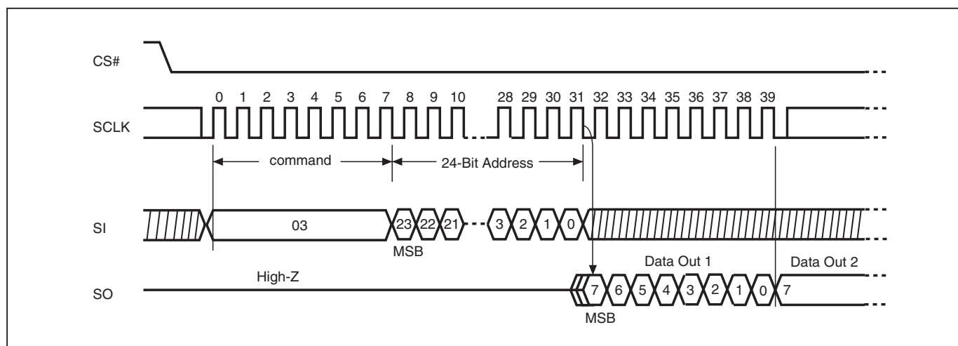
Figure 16. Read Data Bytes (READ) Sequence (Command 03)
