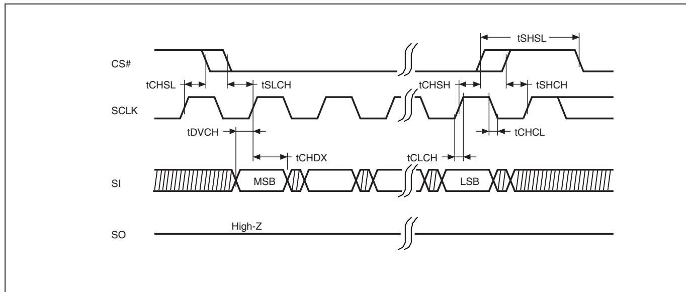
Figure 7. Serial Input Timing
