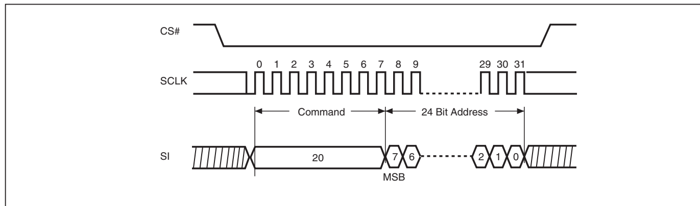
Figure 19. Sector Erase (SE) Sequence (Command 20)
