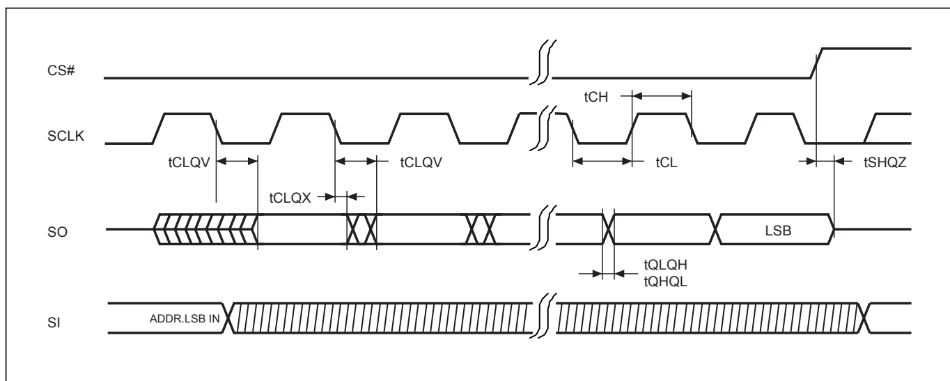
Figure 8. Output Timing
