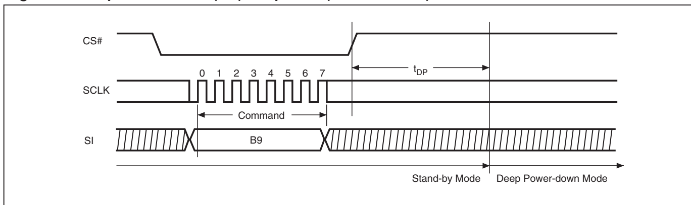
Figure 22. Deep Power-down (DP) Sequence (Command B9)
