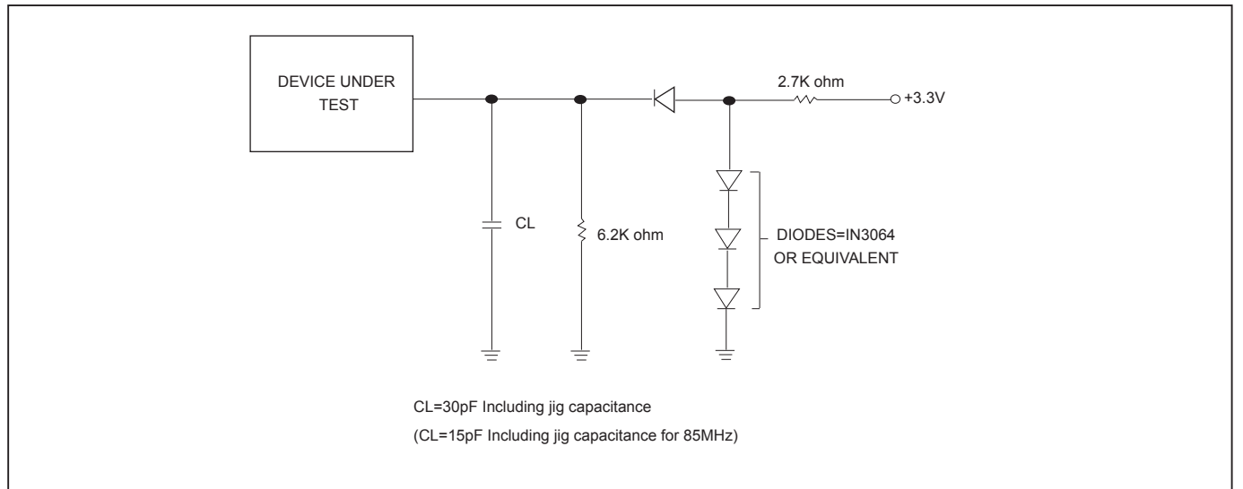
Figure 6. OUTPUT LOADING
