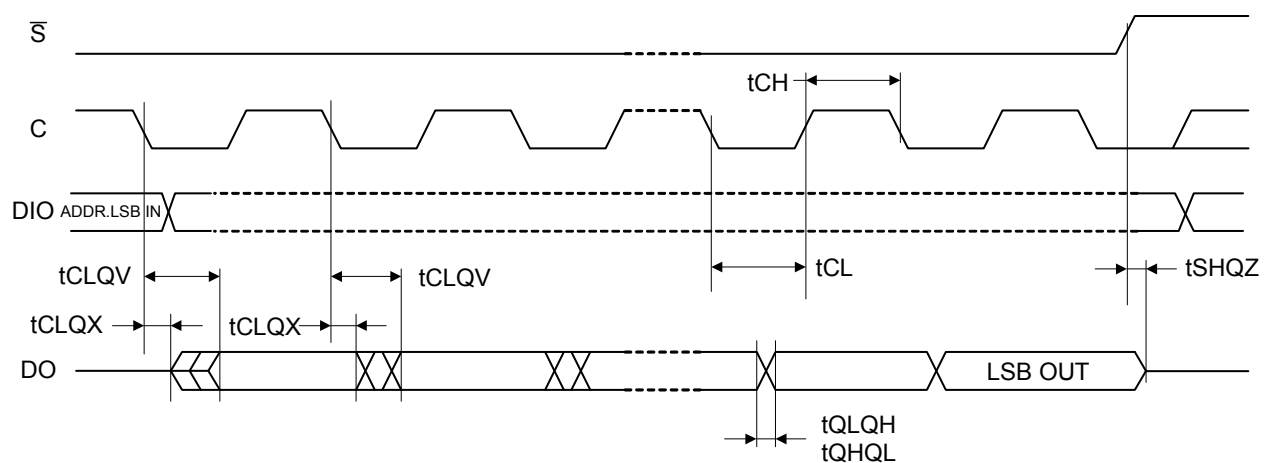
Figure 26. Output Timing
