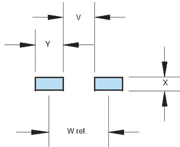
Land Pattern
