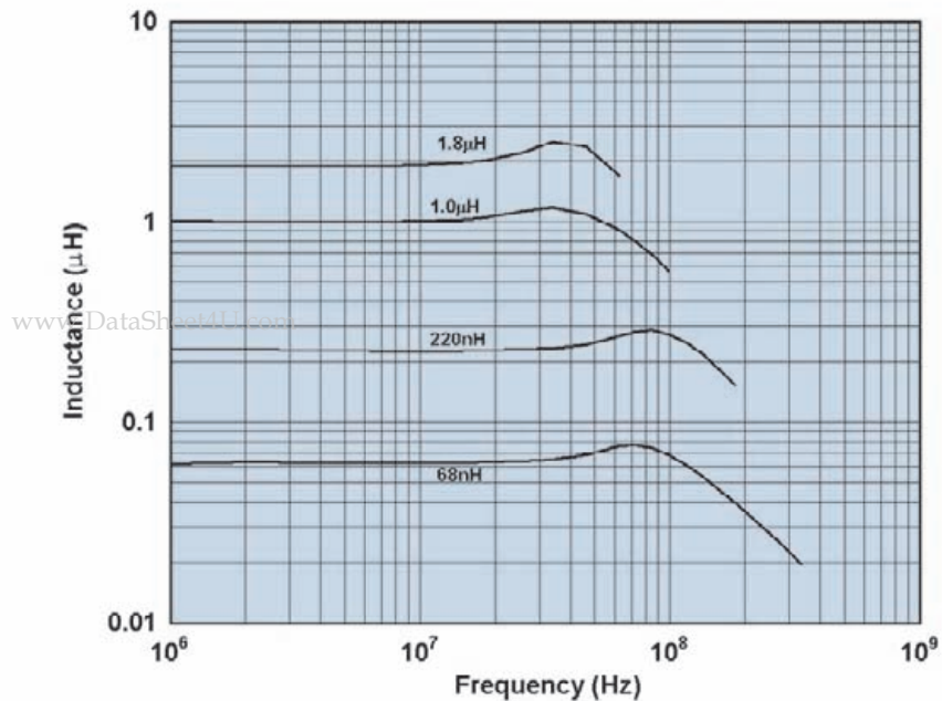
Inductance vs. Frequency
