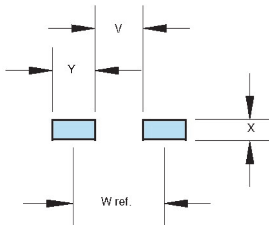
Land Pattern
