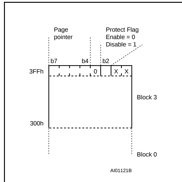
Figure 7. Memory Protection
