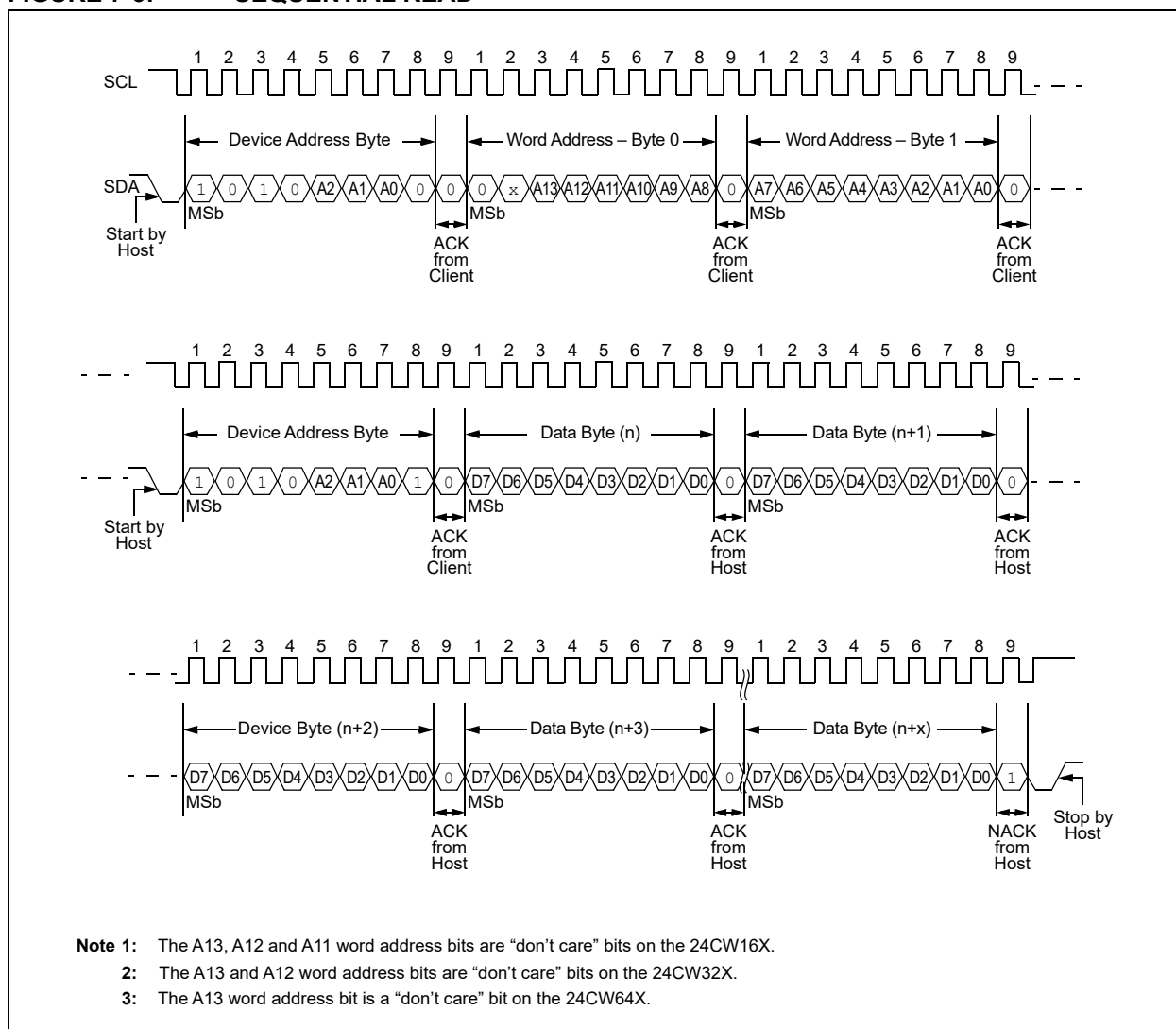
FIGURE 7-3: SEQUENTIAL READ
