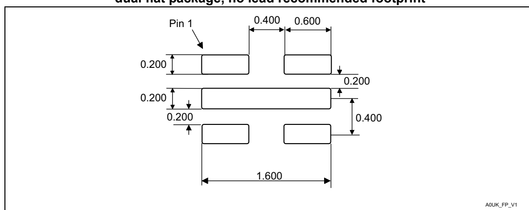
Figure 19. UDFPN5 - 5-lead, 1.7 × 1.4 mm, 0.55 mm thickness, ultra thin fine pitch dual flat package, no lead recommended footprint
