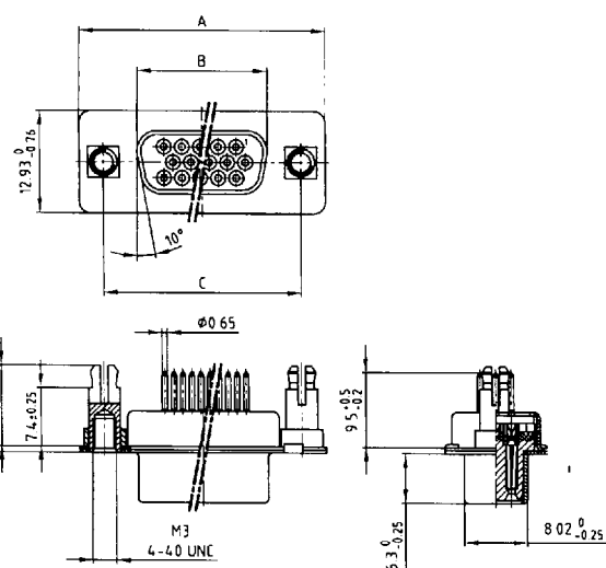
Socket connector
