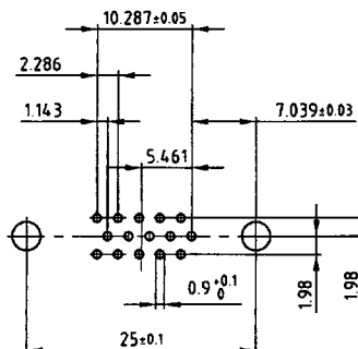
15 pos Socket connector solder pin straight
