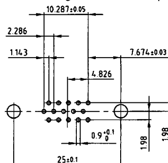
15 pos Plug connector solder pin straight
