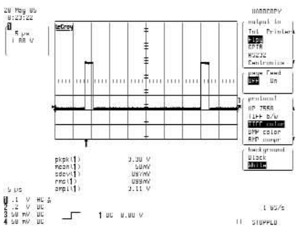
Ref.8 HDMI V Signal output : IC600, #3
