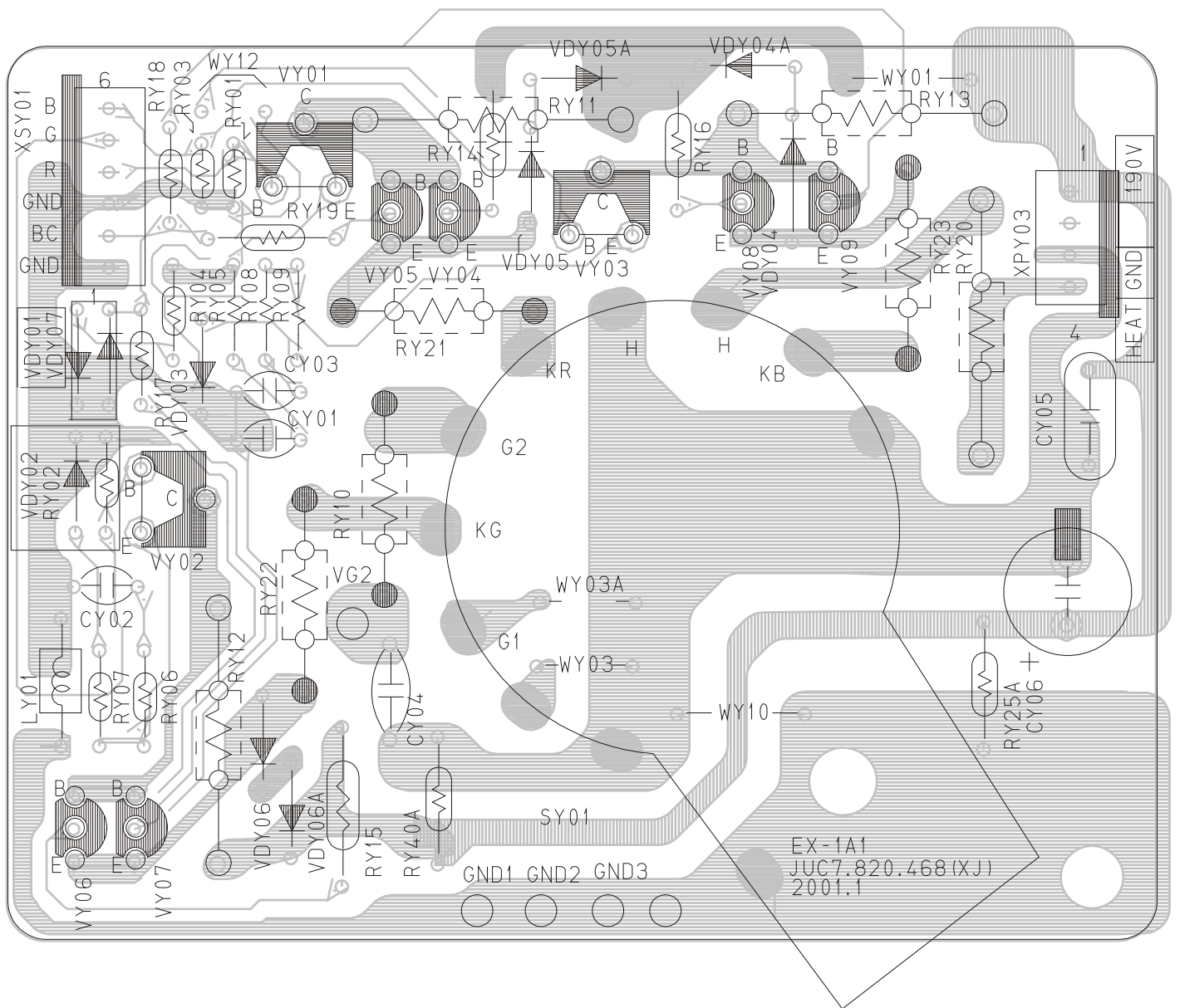
CRT RGB PCB FOR 21NF55/21PF93
