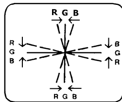
Incline the Yoke up (or down)
