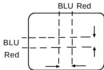
4-pole Magnet Movement
