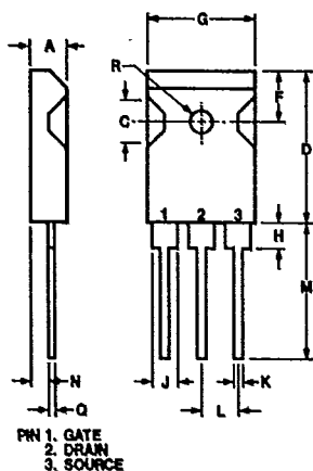
TO-247 (3 LEADED)
