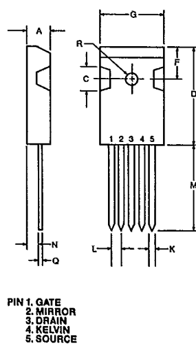
TO-247 (5 LEADED)
