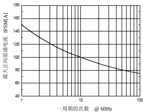
6. Non-Repetitive Surge Current (per diode)
