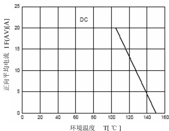
5. Forward Current Derating Curve
