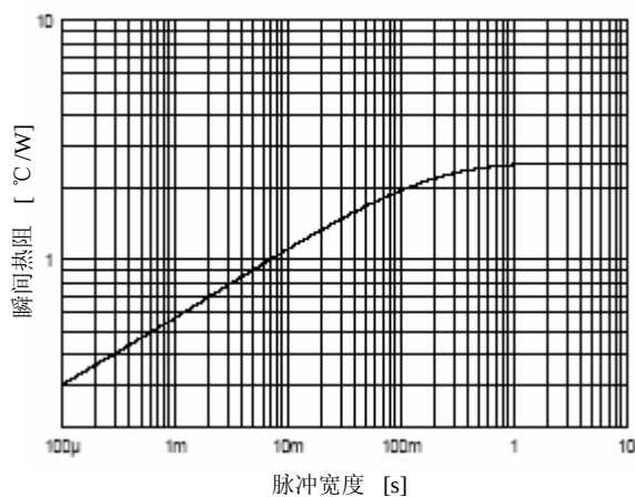
4. Thermal Impedance Characteristics (per diode)
