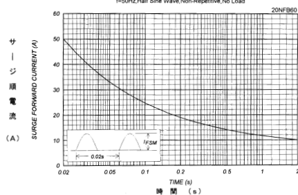
FIG.5 サーージ順電流定格 SURGE CURRENT RATINGS f=50Hz, Half Sine Wave, Non-Repetitive, No Load
