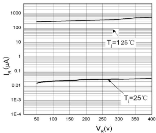
I_R vs V_R
