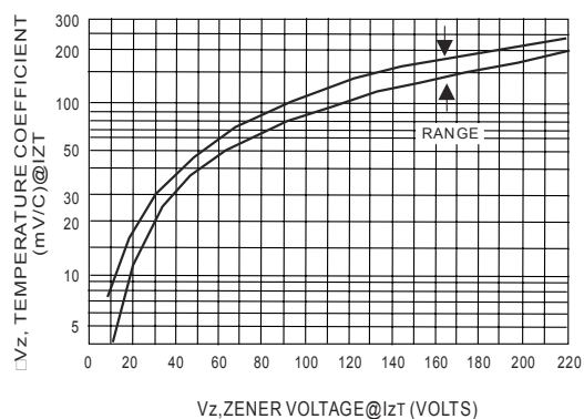
Fig.2 Temperature Coefficient-Range for Units 11 to 39 Volts
