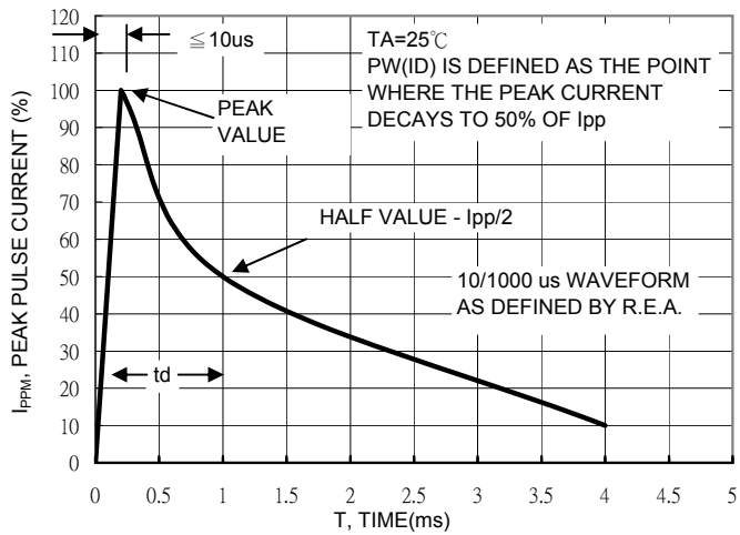
FIG. 7 PULSE WAVEFORM
