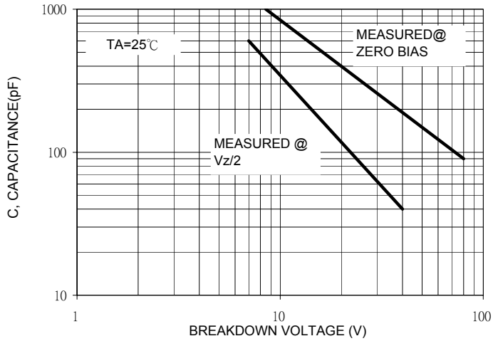
FIG.5 CAPACITANCE CURVE
