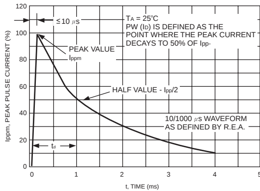
FIG.7- PULSE WAVEFORM
