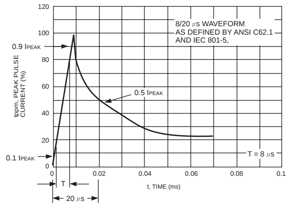
FIG.8- PULSE WAVEFORM
