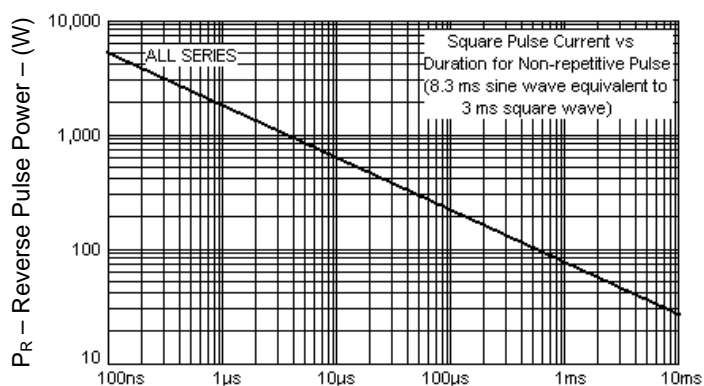
Pulse Duration
