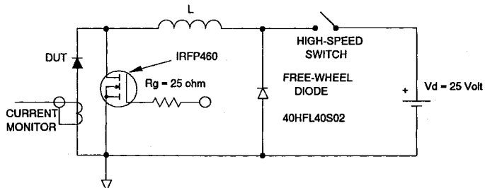
Fig. 8 - Unclamped Inductive Test Circuit
