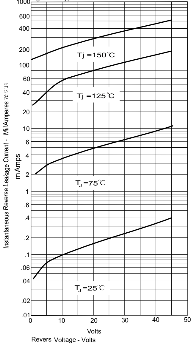
Figure .4- Typical Reverse Characteristics
